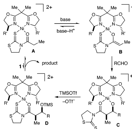
Scheme 1. Proposed Catalytic Cycle
