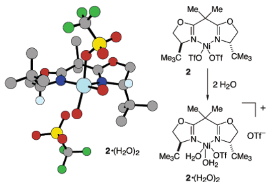
Figure 1. X-ray structure of [Ni(( S,S )- t -BuBox)](OTf) 2 · 2(H 2 O) 2 .
